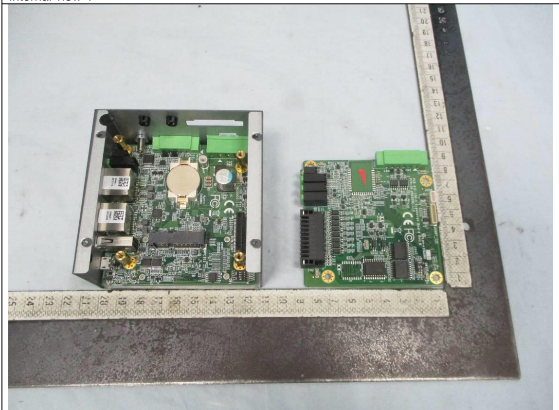
Internal view-2
