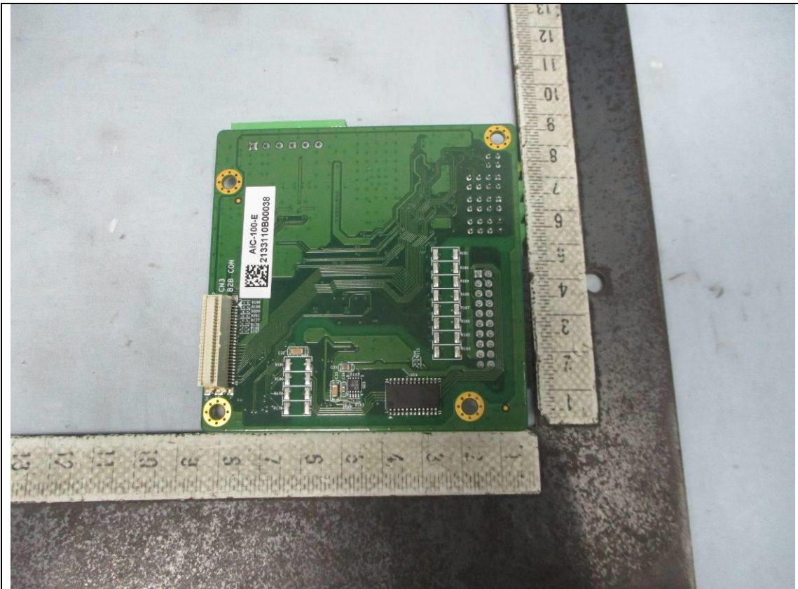
Bottom side view of Isolated board
